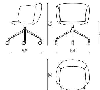
NT 5090 aluminum base armchair on casters
